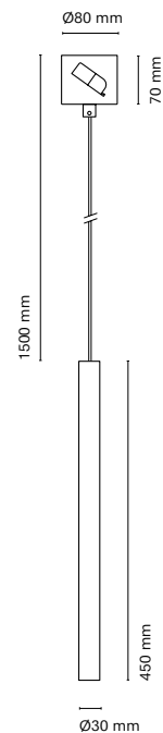
06753- Bcn 30 Air 450 mm (Canopy)
